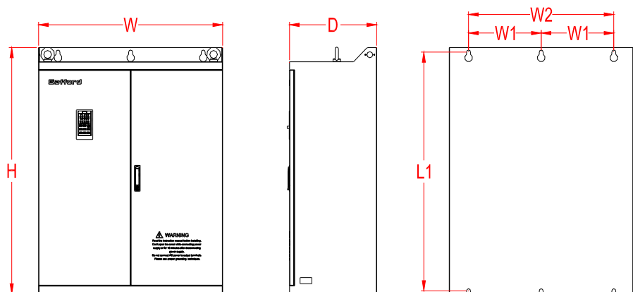
GD600 450G-630G 壁挂机外型及安装孔位尺寸
