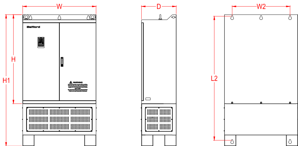
GD600 450G-630G 壁挂机加底座外型及安装孔位尺寸
