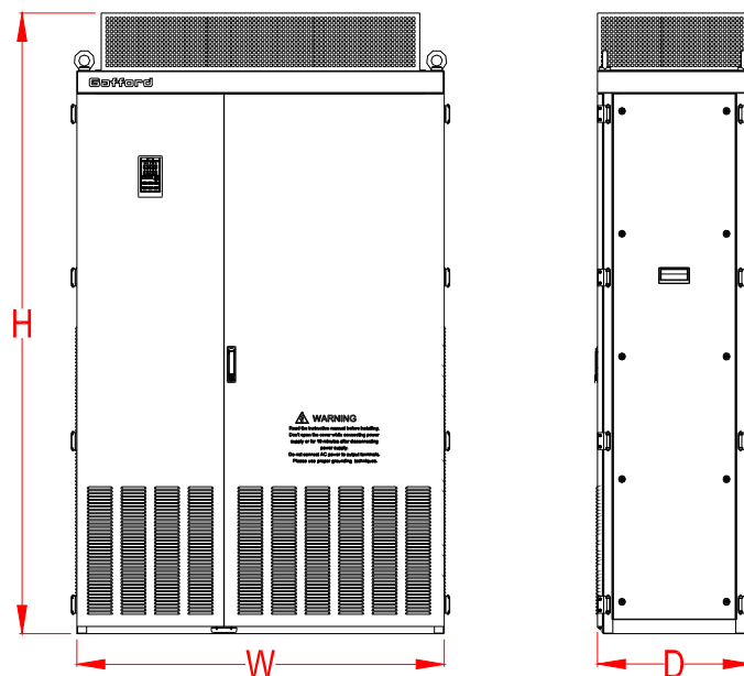
GD600 710G-900G 柜机外型及安装孔位尺寸
